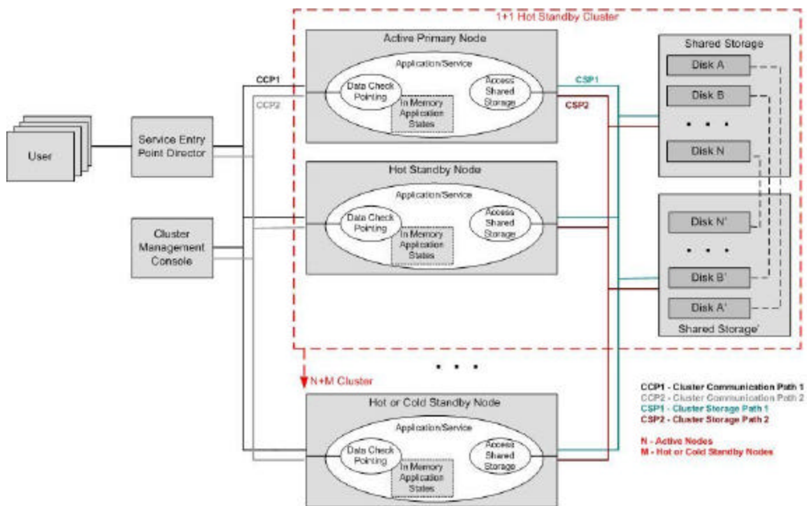
Illustration 2. CGL Cluster Model
