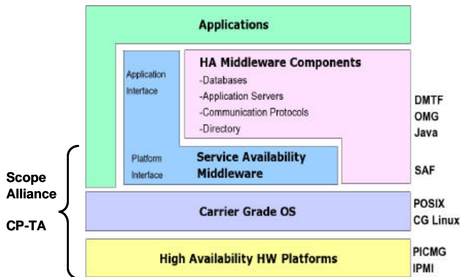
Illustration 2: Full Carrier Grade Application Stack
